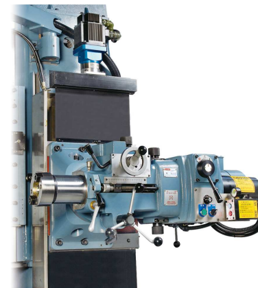
HK砲塔式主軸(主軸可伸縮) HK Turret Type Spindle (Over Travel 140mm)
